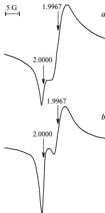
Fig. 1. ESR spectra of a frozen solution of the C_{60}^{\bullet-} radical monoanion ( C_{60} with KOH in BN) before ( a ) and after storage in the air for 20 min ( b ).
