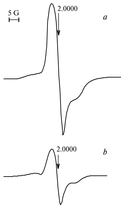
Fig. 2. ESR spectra of a frozen solution of the C 60 2- dianion (C 60 with Mg/KOH in DMF) before (a) and after storage in air for 20 min (b).
