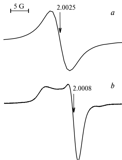
Fig. 3. ESR spectra of a frozen solution of the C 60 •3- radical trianion (C 60 with Zn/KOH in DMF) before (a) and after storage in air for 20 min (b).
